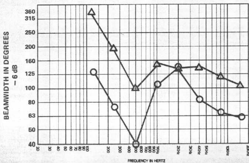
FIGURE 3 Dominator Beamwidth vs. Frequency (System Long-Axis Vertical)
